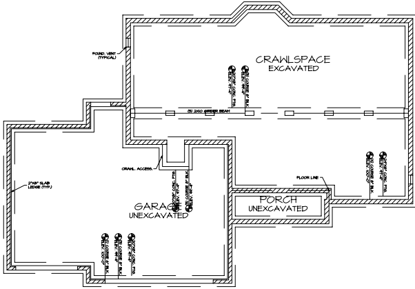
FOUNDATION PLAN A-3 SCALE: 1/4"=1'-0"
