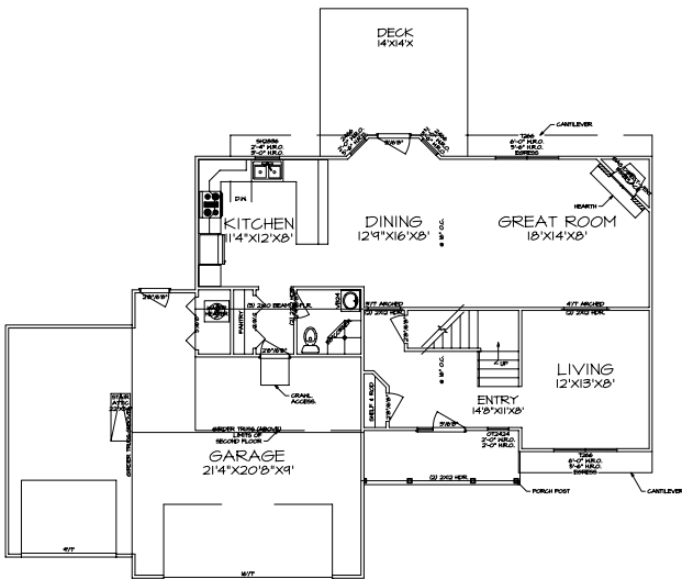
FIRST FLOOR PLAN A-4 SCALE: 1/4"=1'-0"
