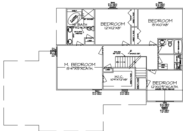
SECOND FLOOR PLAN A-5 SCALE: 1/4"=1'-0"
